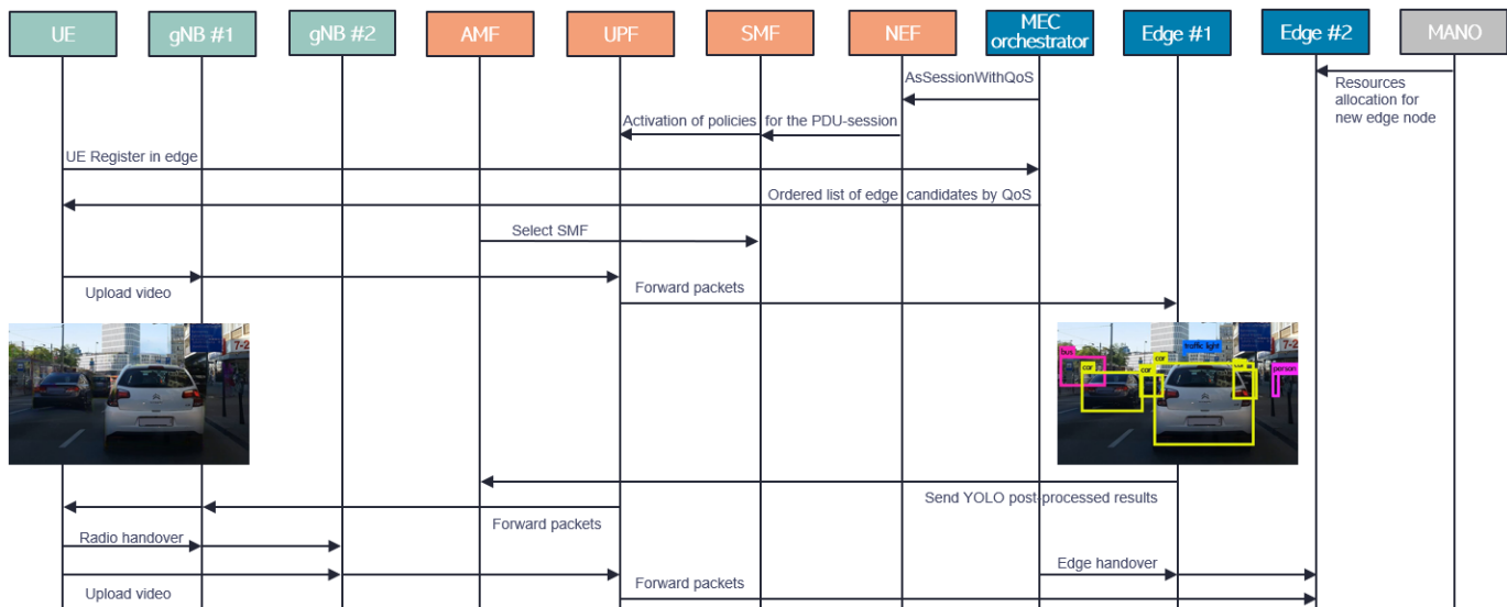
Fig. 2. Call-flow diagram
